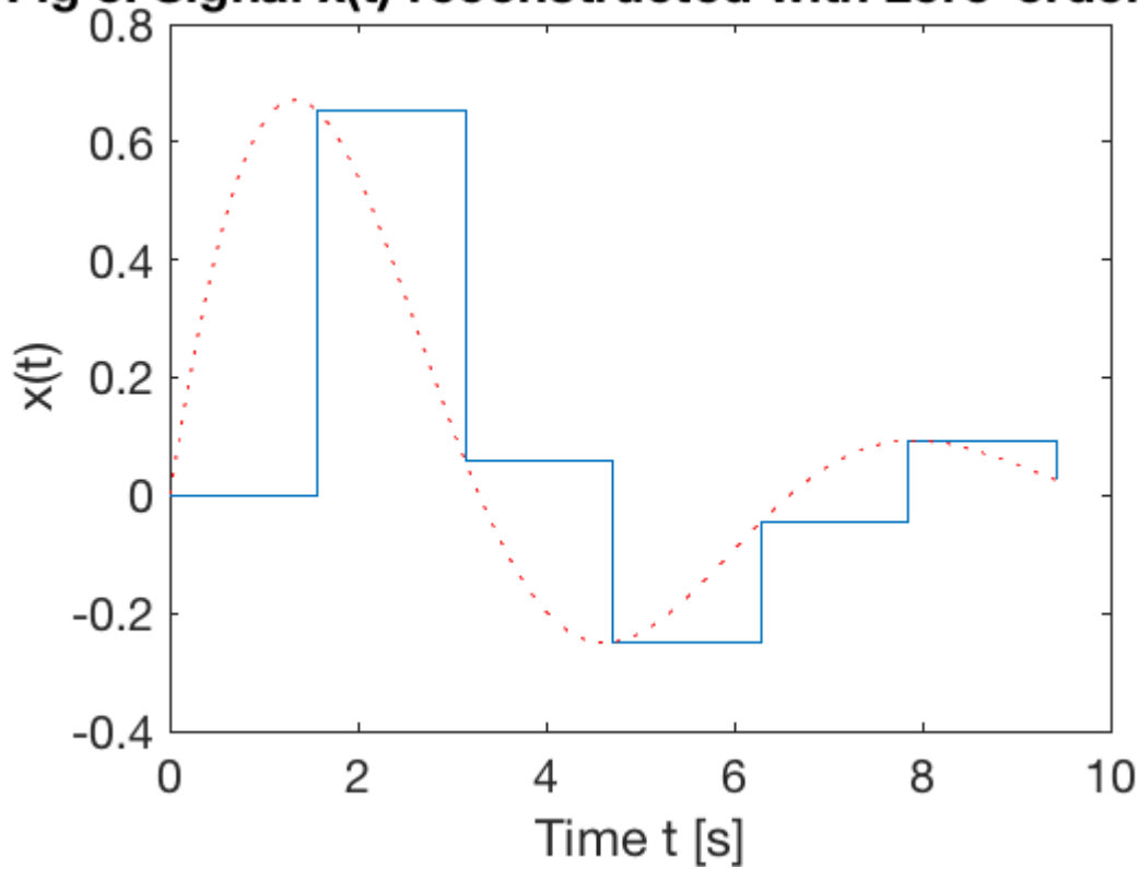
Fig 3: Signal x(t) reconstructed with zero-order-ho
